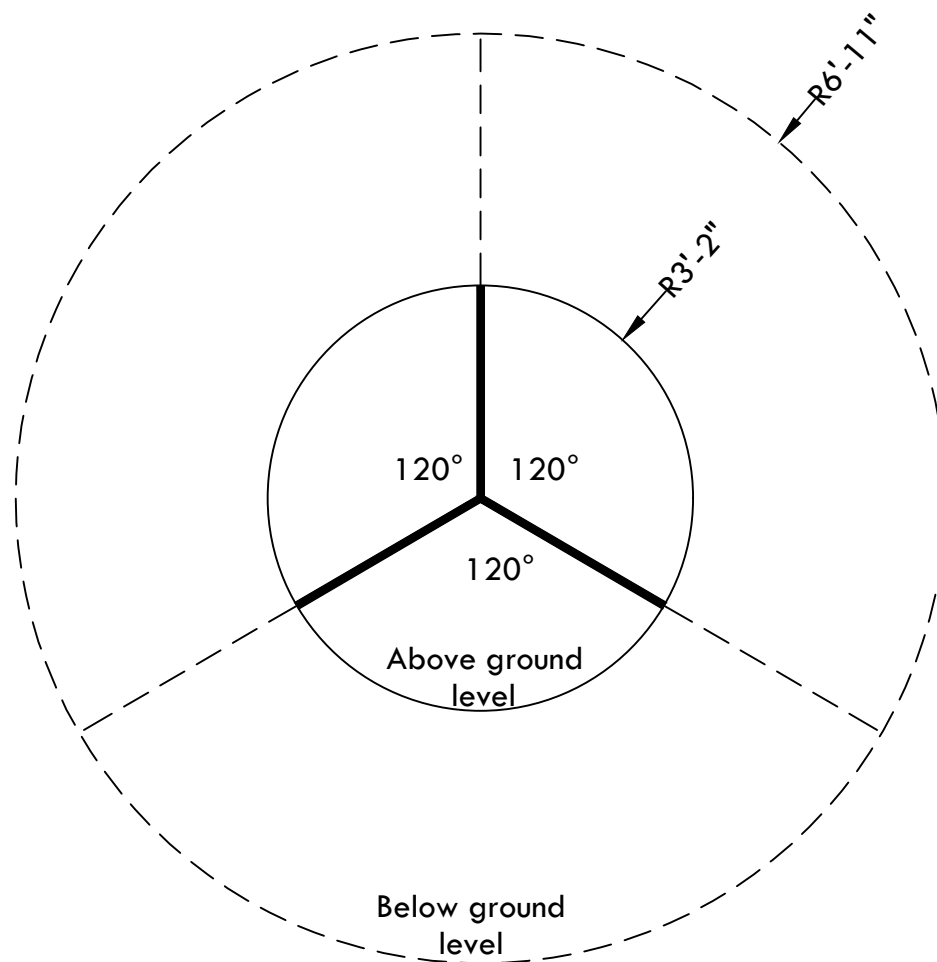
TOP VIEW OF CORS MONUMENT
